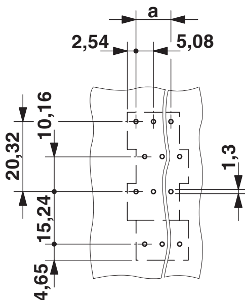
Dimensional drawing
