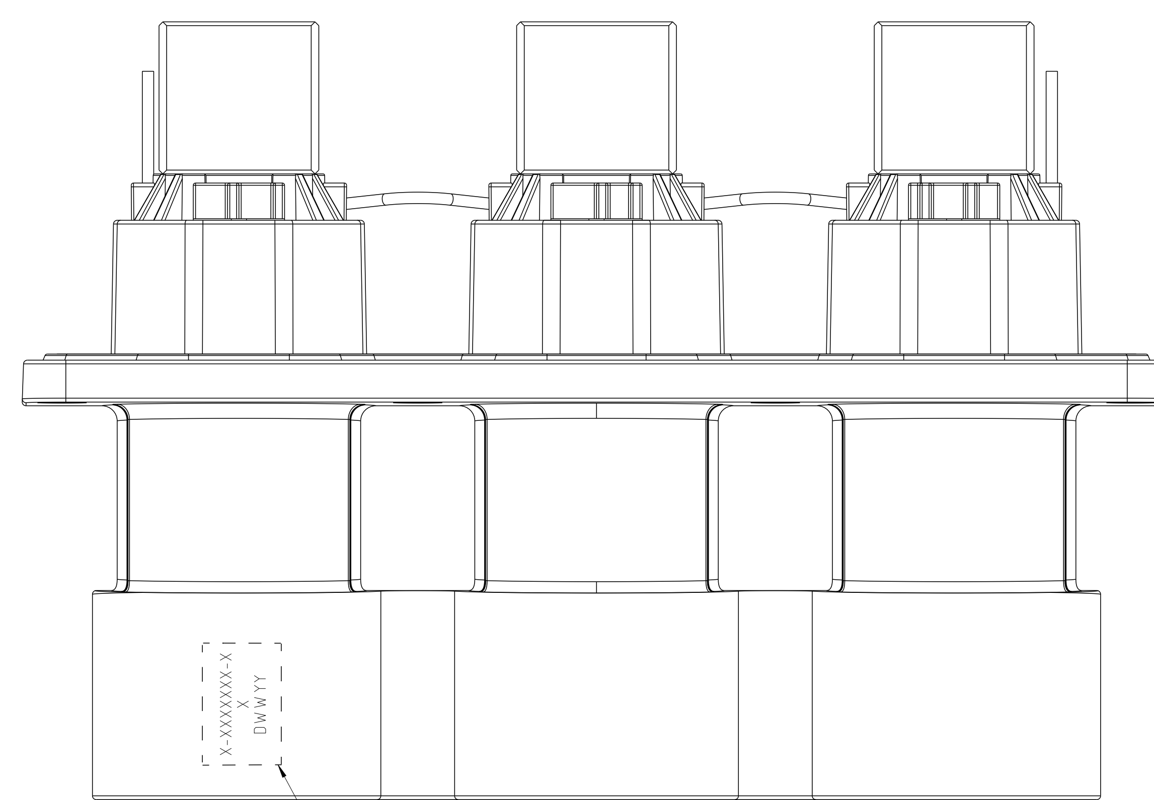
SECTION B-B
