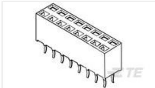
TE Part # 1-215309-7 2X17P HV100 REC CON. TE, 8.5MM
