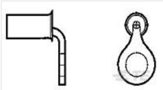
TE Part #55654-1 TERMINAL R 90 DEG PG 8 10
