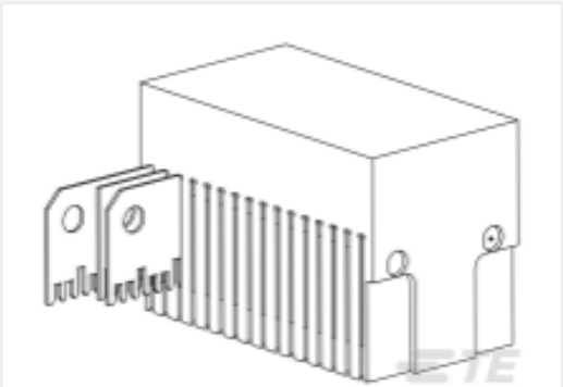
TE Part #1804790-3 SEATING TL ASSY, STD, 4 PAIR
