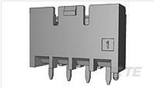
TE Part #3-1376383-4 5MM POWER KEY 3P HDR ASSY YELL
