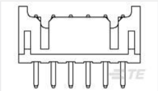
TE Part #2-1470109-2 2.0mm Pitch Header, Dip 22p
