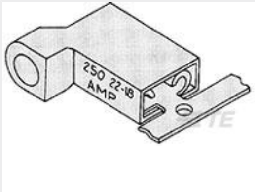
TE Part #3-520340-2 ULTRA-FAST 187 ASY REC 16-14 AWG TPBR
