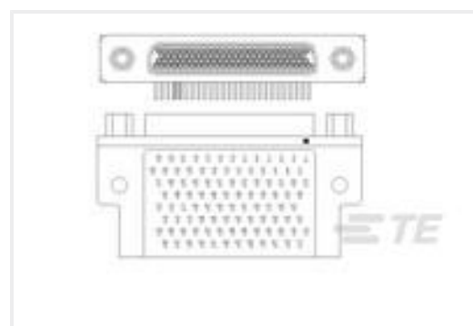
TE Part #1532257-4 M83513/12-H01NP = MCKS-N1-S-100PRT1
