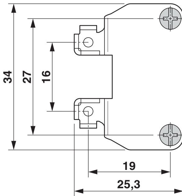
Dimensional drawing
