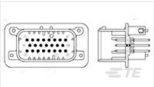
TE Part #776228-5 23POS,PIN DIA 1.3,HDR ASSY, 180DEG,COD 5
