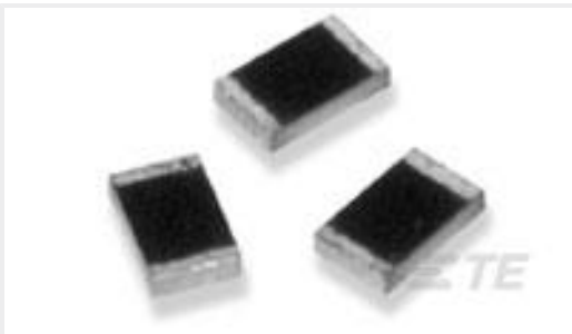
TE Part #1879808-1 RP 1J 1K0 0.1% 15PPM 5K RL
