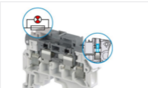
TE Part #1SNK508413R0000 ZS4-SF1-R2
