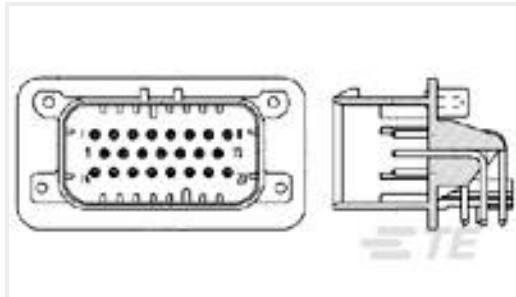
TE Part #1-776087-1 23POS,PIN DIA 1.3,HDR ASSY,90DEG, COD 1
