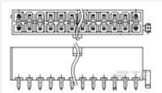
TE Part #3-1775099-3 ATX PWR CONN 1 BDLK 10 POS
