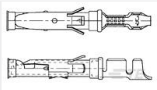
TE Part #163092-2 .062 DIA SOCKET ASSY 3+ (LP)
