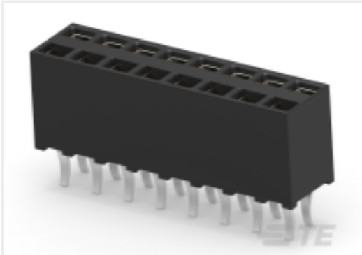
TE Part # 215307-8 2X8P HV100 REC CON. TE, 7.0MM
