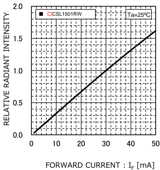
Fig.3 RADIANT Intensity - Forward Current
