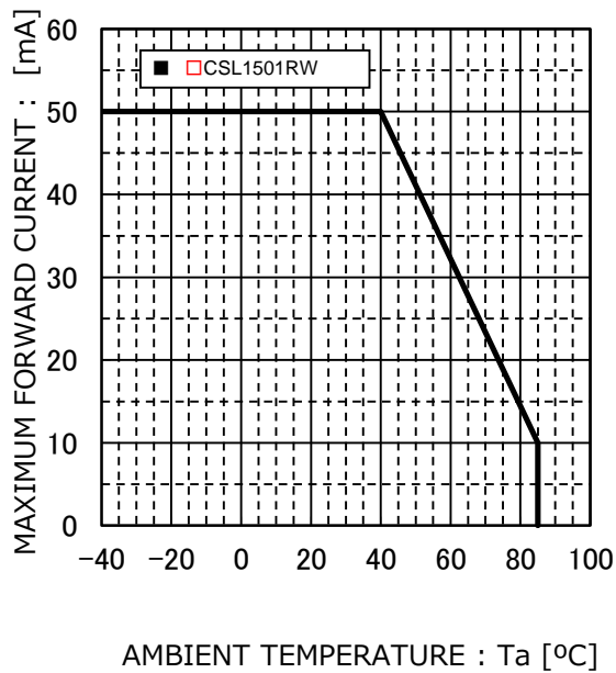
Fig.4 Derating
