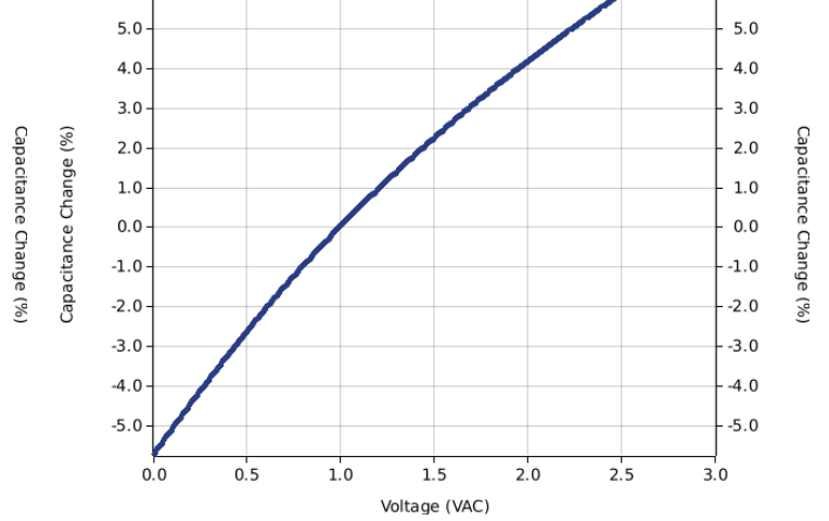
Capacitance Change versus AC Voltage
