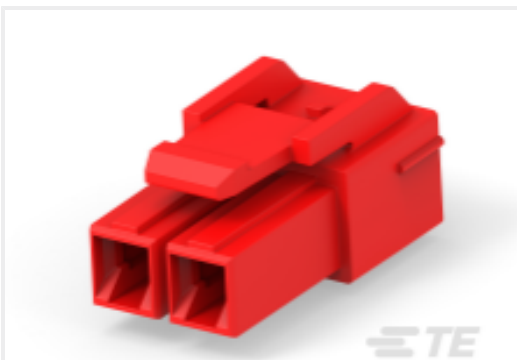
TE Part #1-2408780-2 Plug HSG 2P Red HCI 6.2 Pitch Inner Lock
