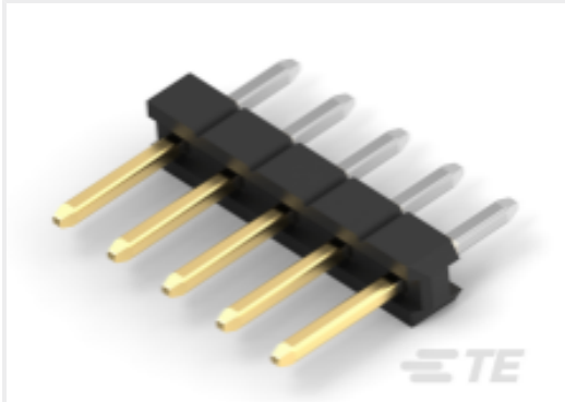
TE Part # 2355181-5 5P,2MM,BRK HDR,SRVT,2.8,0.38AU, BOX
