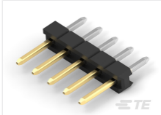
TE Part # 2355177-5 5P,2MM,BRK HDR,SRVT,2.8,0.38AU,TB
