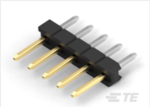
TE Part # 2355179-5 5P,2MM,BRK HDR,SRVT,2.8,0.38AU,TB W/CAP
