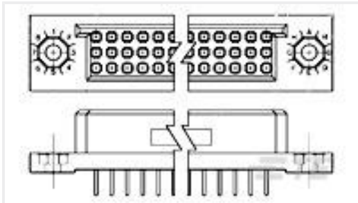
TE Part #533495-3 BOX II 3 ROW RECP ASSY 174 POS
