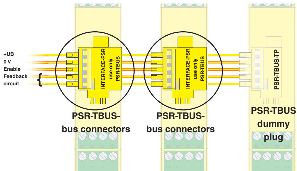
Connection diagram
