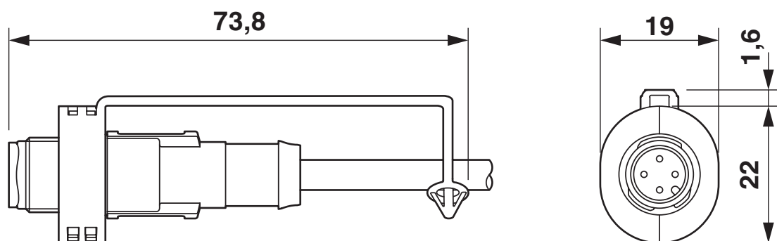
Dimensional drawing
