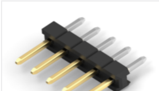
TE Part #2355177-6 6P,2MM,BRK HDR,SRVT,2.8,0.38AU,TB
