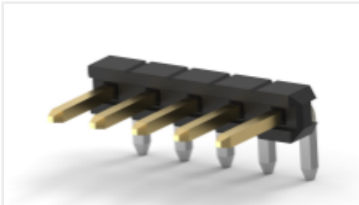
TE Part #2842124-5 5P,2MM,BRK HDR,SRRT,2.8,0.76AU, BOX
