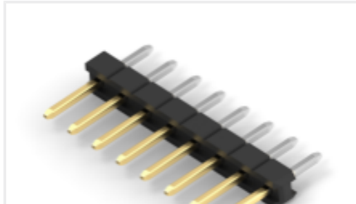
TE Part #2355179-8 8P,2MM,BRK HDR,SRVT,2.8,0.38AU,TB W/CAP
