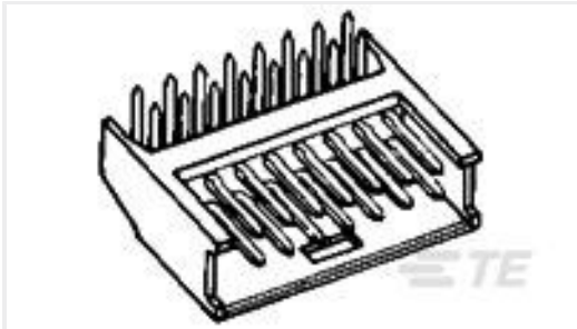
TE Part #280390-1 2X8P MODU II SHRD HDR, RT ANG, TIN
