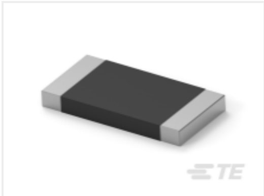
TE Part #3-2176422-1 TLRP 2512 3.0W R047 1% 25PPM 4K RL
