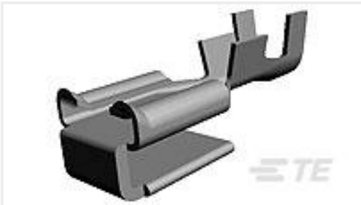
TE Part #62109-2 250 FASTON REC 18-14 AWG TPBR
