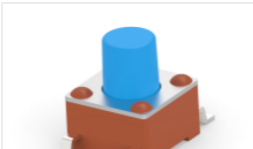
TE Part #1-1977223-6 FSM6JSMLSTR=6MM TACT SWITCH, SMT 100gf,
