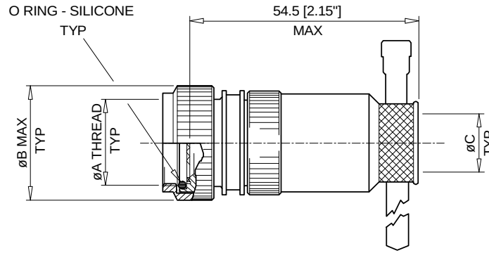
STRAIGHT ADAPTOR -00
