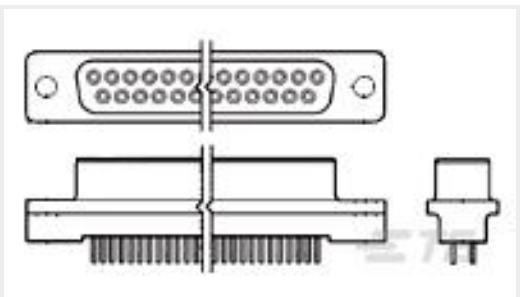
TE Part #5207826-3 HD-20 RCPT 9P VERT
