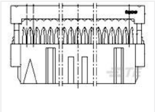
TE Part #6-215882-4 64 WAY GREY MK II RECP
