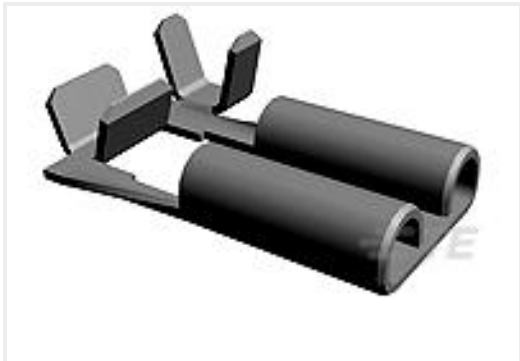
TE Part #1742089-2 187 FASTON,FLAG,REC.,18-14OR2X18AWG,TPBR
