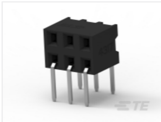
TE Part # 2307718-6 6P,2MM,B-B,REC,DRHZ,2.1,0.38AU,TR
