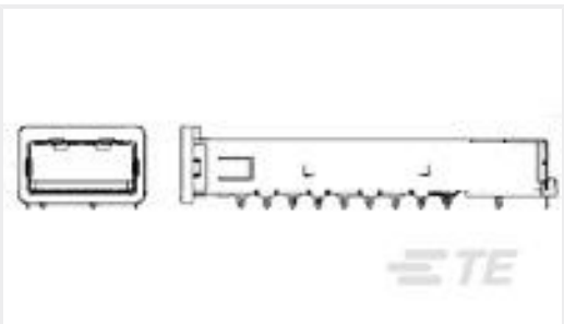
TE Part #1888101-1 XFP CAGE ASSEMBLY w/o Elastomeric Gasket
