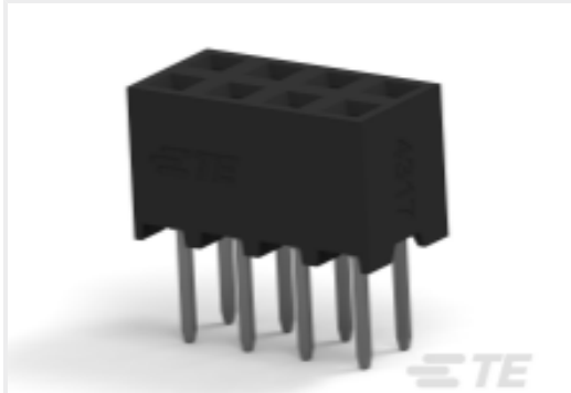
TE Part # 2307785-8 8P,2MM,B-B,REC,DRV,T,2.0,0.76AU,TR, W/CAP
