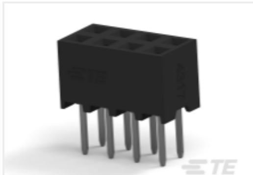
TE Part # 2314822-8 8P,2MM,B-B,REC,DRV,T,2.7,0.76AU,TB
