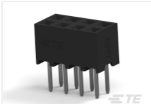
TE Part # 2314814-8 8P,2MM,B-B,REC,DRV,T,2.0,0.76AU,TB, W/CAP
