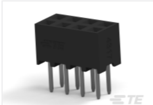
TE Part # 2307786-8 8P,2MM,B-B,REC,DRV,T,2.7,0.76AU,TR, W/CAP
