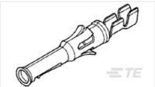
TE Part #350561-7 UMNL PIN 24-18 .0126 AU/Ni/BR
