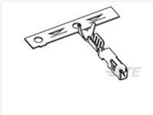
TE Part #1924955-1 CONTACT,FEMALE0.64,20-22AWG, UNSEAL
