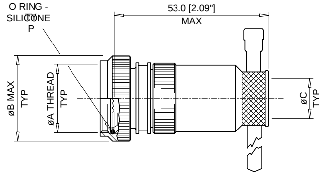
STRAIGHT ADAPTOR -00
