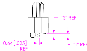
FIG 3 -DS WITH -L OPTION (-DS AVAILABLE ON -05.0 LEADSTYLE ONLY) (-L AVAILABLE ON -05.0 & -09.0 LEAD STYLE ONLY) (ERM8-025-05.0-XXX-DV-DS-L SHOWN) (SAME AS FIG 1, EXCEPT AS SHOWN) (SOME CENTER FEATURES REMOVED FOR CLARITY)
