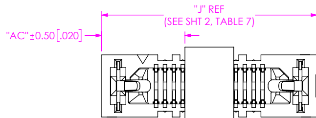
FIG 10 -P WITH -L OPTION (ERM8-013-XX.X-XXX-DV-L-P SHOWN) (SAME AS FIG 9, EXCEPT AS SHOWN) (SOME CENTER FEATURES REMOVED FOR CLARITY)
