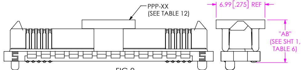
FIG 9 -P OPTION (ERM8-030-XX.X-XXX-DV-P SHOWN) (SAME AS FIG 1, EXCEPT AS SHOWN) (SOME CENTER FEATURES REMOVED FOR CLARITY)
