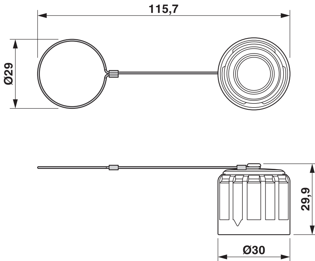
Dimensional drawing
