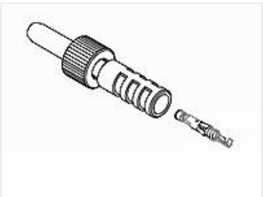
TE Part #5-861610-3 LGH, HIGH VOLTAGE PLUG
