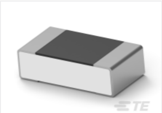
TE Part #9-2176371-6 RQ 0603 45K3 0.1% 10PPM 5K RL
