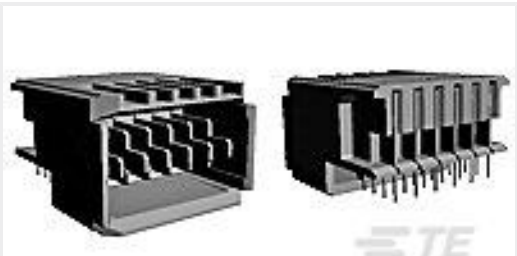
TE Part #2000713-6 RA Keyed Guide Mod, Vita 46, Machined
