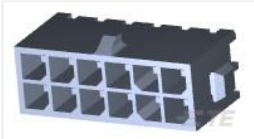
TE Part #4-794632-2 12P MICRO MNL ASSY,VRT,HDR,LF
