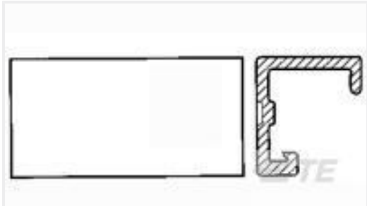
TE Part #1-640550-2 12P MTA100 COVER
