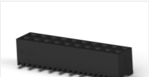
TE Part #2-2314844-0 20P,2MM,B-B,REC,DRVT,SMD,0.1AU, TB,W/CP
