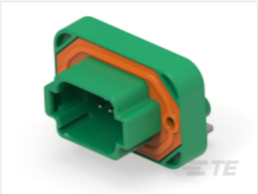
TE Part #DT13-08PC HDR, 8P, GRN, RA, NI/CU, C
