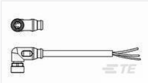
TE Part #1-2273011-1 M8 x 1.0 Angled socket Pigtail
