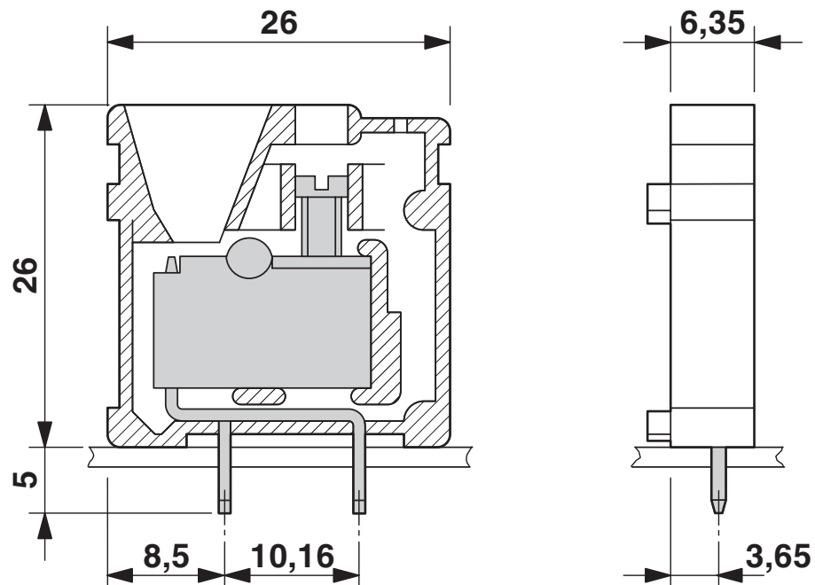
Dimensional drawing
