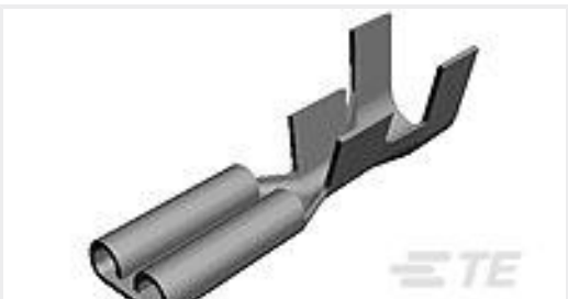
TE Part #42640-1 250 FASTON REC 22-18 AWG BR
