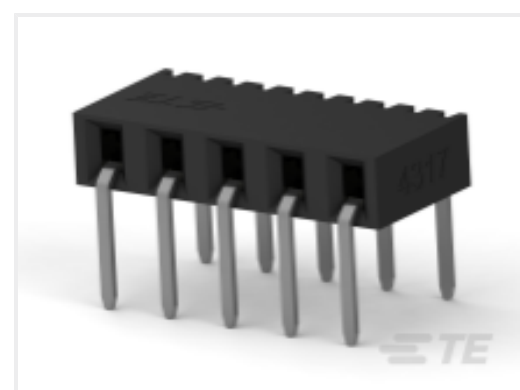
TE Part # 2307708-4 4P,2MM,B-B,REC,SRHZ,3.4,0.38AU, TUBE
