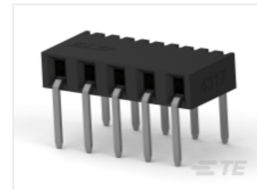
TE Part # 2314937-4 4P,2MM,B-B,REC,SRHZ,2.8,0.38AU,TR
