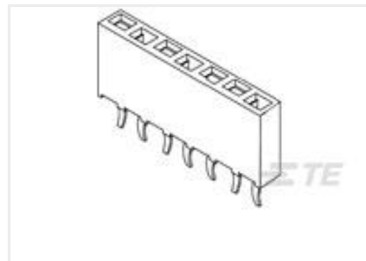
TE Part #1-215297-1 11P HV100 REC CON. TE, 7.0MM
