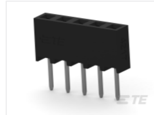
TE Part # 2314877-4 4P,2MM,B-B,REC,SRVT,2.7,0.38AU,TB
