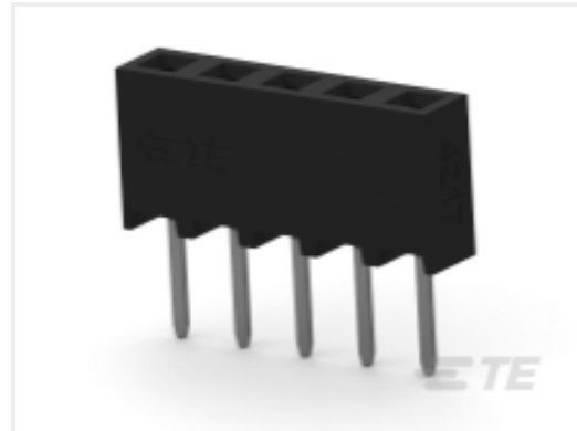
TE Part # 2314869-4 4P,2MM,BB,REC,SRVT,2.0,0.38AU,TB, W/CAP
