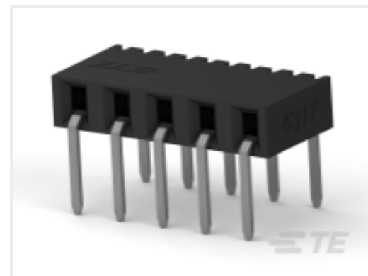
TE Part # 2307707-4 4P,2MM,B-B,REC,SRHZ,2.8,0.38AU,TB
