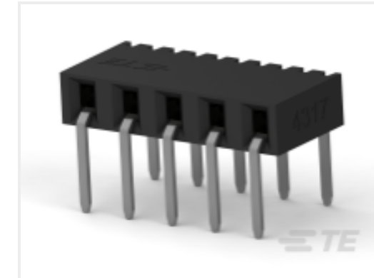
TE Part # 2314929-4 4P,2MM,B-B,REC,SRHZ,2.1,0.38AU,TB
