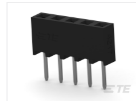
TE Part # 2314881-4 4P,2MM,BB,REC,SRVT,2.7,0.38AU,TB, W/CP
