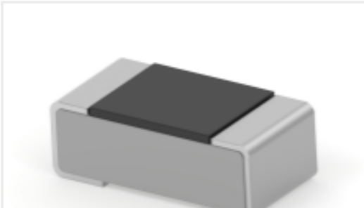
TE Part #4-2176338-3 CRGCQ 0402 10M 5%
